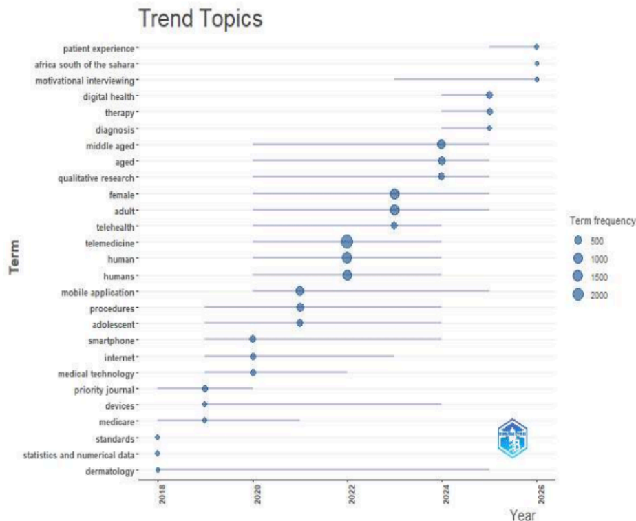
Figure 5. Trend Topics
